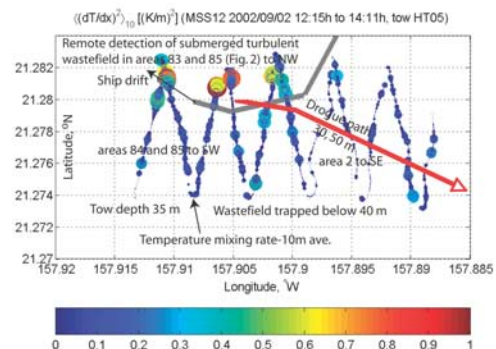
Figure 6. Circle sizes and colors indicate 10-m averages of temperature gradient variance \sigma(T_x) = \langle\langle (dT/dx)^2 \rangle\rangle along a towpath above the 40–50 trapping depth, at \sim 35 m.
