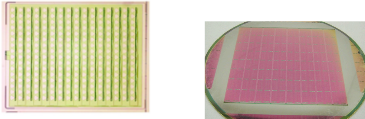
Figure 3: On the left is a MKID demonstration array. On the right is a planar phased array of antennas coupled to detectors. Each of the 64 elements measures both polarizations. Multiple sub arrays may be combined. Both of these examples are from Caltech/JPL.
