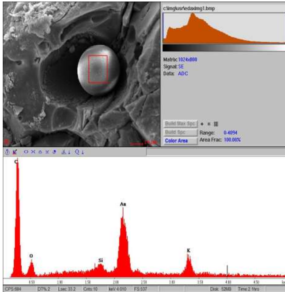
Fig.2 Microsphere held in a cavity within the Polonnaruwa meteorite together with EDX showing analysis showing its carbonaceous composition.
