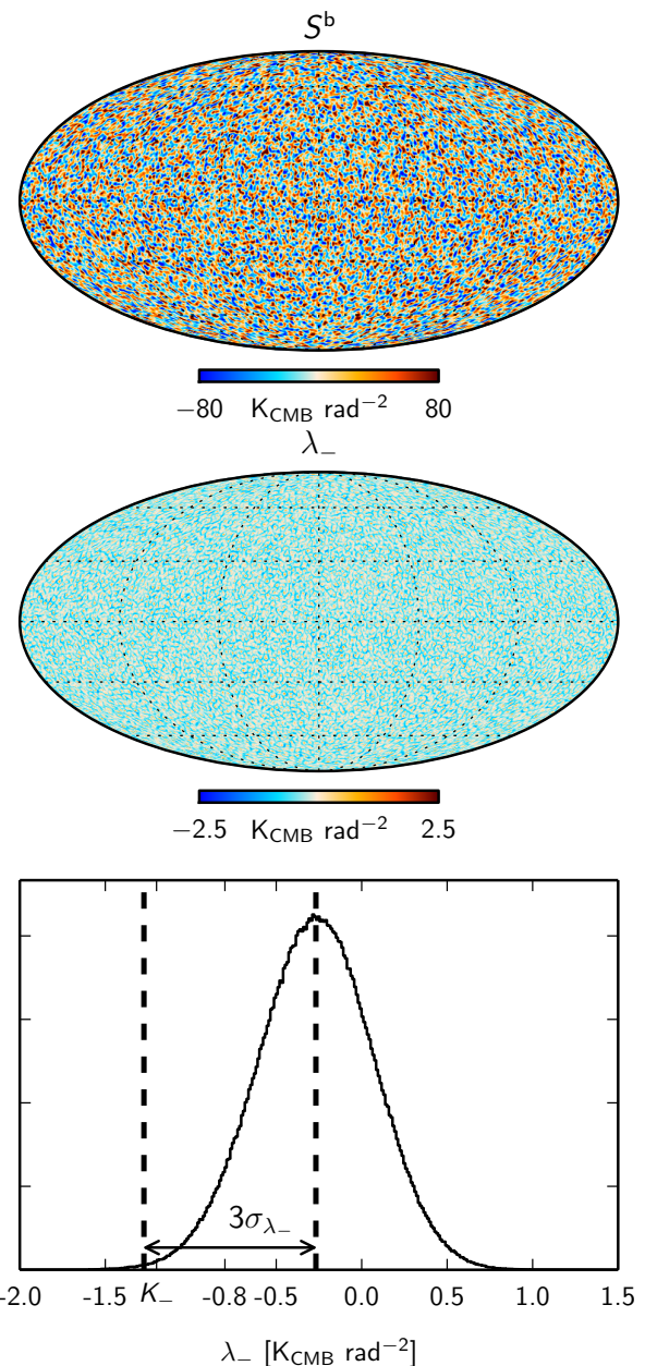
Fig. A.1. Filtered realization of the Gaussian dust sky (upper panel) and the corresponding eigenvalue \lambda_- (middle panel). The distribution of the eigenvalue \lambda_- (lower panel) over the unmasked pixels is Gaussian.
