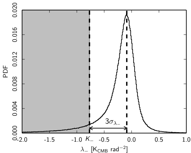
Fig. 3. Distribution of the eigenvalues \lambda_- over the unmasked pixels in the high-latitude sky. The grey region represents the pixels that were used in the SMAFF algorithm to find strong filaments.
