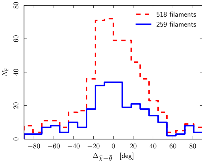
Fig. C.1. Same as the upper panel of Fig. 6, when including angle differences \Delta\bar{\chi}_- - \bar{\theta}_- from the weak filaments. The width of the histogram does not change.
