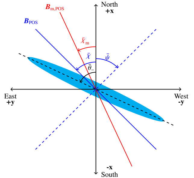
Fig. 5. Sketch of the mean orientation angle of the filament ( \bar{\theta}_- ), the magnetic field ( \chi ), the polarization angle ( \psi ), and the large-scale GMF ( \bar{\chi}_m ) along the filament. All the angles are defined with respect to the GN and follow the IAU convention.
