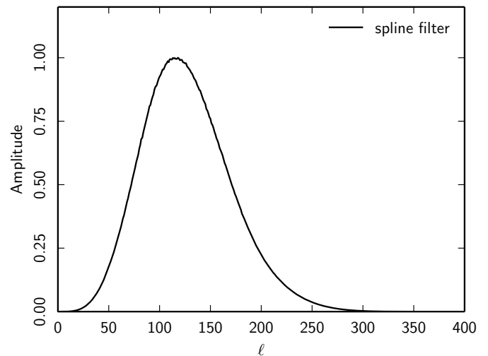
Fig. 1. The representative bandpass filter, retaining only the scales between \ell = 30 and 300.
