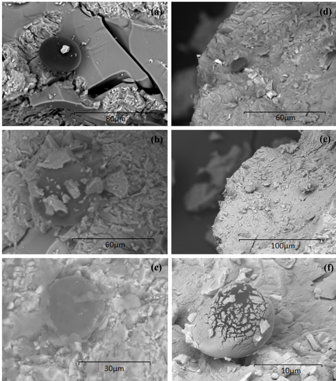
Fig. 1. Scanning electron microscopy images of the Tissint meteorite. (a) An image of a spherical structure found on the first fresh fracture, (b) a similar structure found in a second fresh fracture and on the surface (c). Images (d) – (f) depict a similar structure under different conditions: (d) uncoated, and (e) and (f) show same structure under gold coating. Cracking seen in (f) probably indicates an original C,O rich structure that is hollow.
