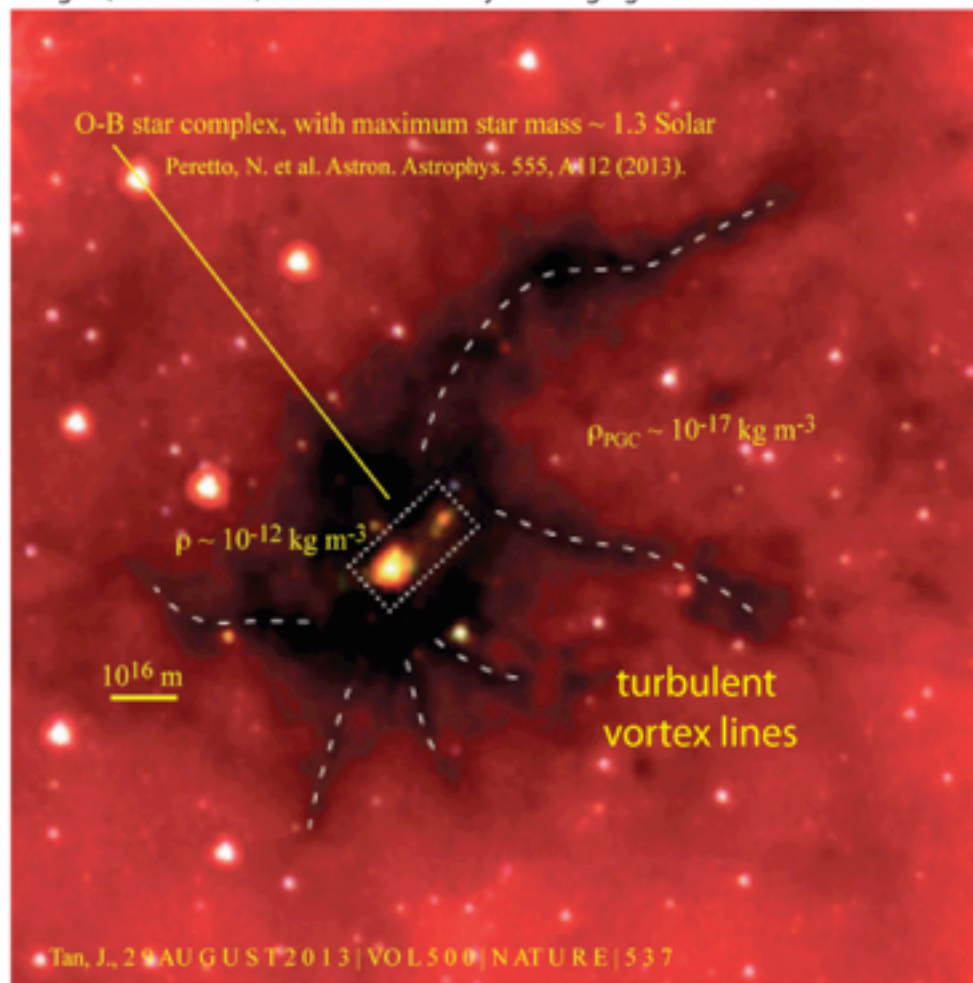
Infrared image from Spitzer Space Telescope shows the SDC 335 dark cloud interior Evidence of rapid O-B star formation by planet fluid turbulence
