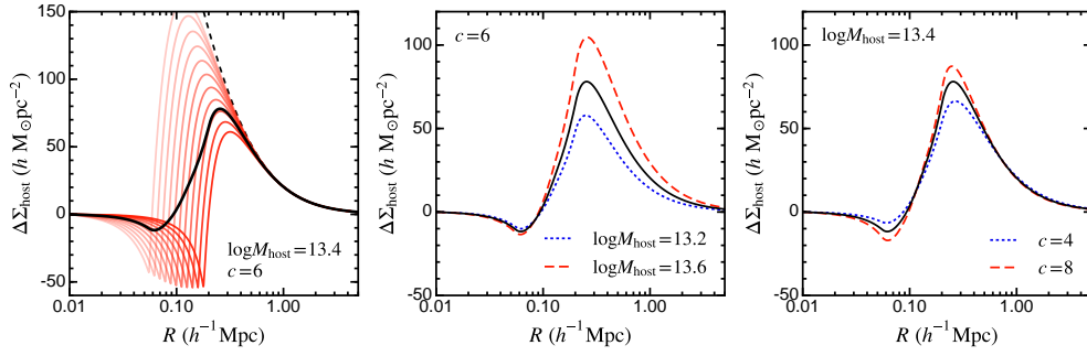
Figure 3. Illustration of the contribution from the host group, \Delta\Sigma_{\text{host}}(R)n(R_{\text{sat}}) , to Equation 7. Left: Red lines show the contribution to the signal around satellites at different distances from the group centre in logarithmic bins, with opacity scaling with the number density of objects in each bin, n(R_{\text{sat}}) , corresponding to the cyan histogram in the top-left panel of Figure 2. The thick black line is the weighted average of the red lines (cf. Equation 12) and represents the group contribution to the lensing signal around our sample of satellites with 0.05 \leq R_{\text{sat}}/(h^{-1}\text{Mpc}) \leq 0.20 in a group with \log M_{200} = 13.4 and c = 6 , and is reproduced in the middle and right panels. The black dashed line shows the excess surface density of the same group when measured around the group centre. Middle: Varying group mass at fixed concentration. Right: Varying group concentration at fixed mass. Note that the vertical scale in the middle and right panels is zoomed in with respect to the left panel. All masses are in units of h^{-1}M_{\odot} .
