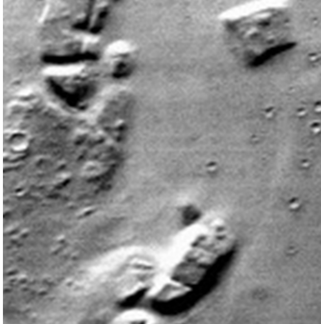
Figure 38. Galaxias Face A “Galaxias” and Galaxias Face B “Chaos” are seen in portion of Odyssey THEMIS Image I02816002
