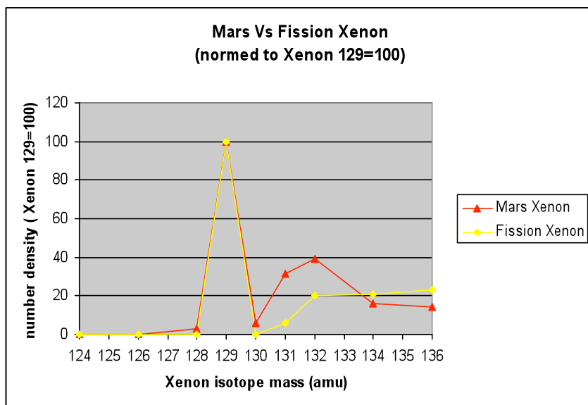
Figure 3. Mars Xenon and Earth Nuclear testing Xe normed to ^{129}\text{Xe} concentration, data taken from [6].
