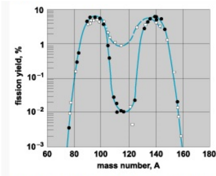
Figure 5. Mass distribution of fission fragments formed by neutron induced fission of ^{235}\text{U} when neutrons have been moderated (solid curve) and fission by 14 MeV fusion neutrons (broken curve) (Spence 1949) showing increase in middle range isotopes for fusion neutrons.
